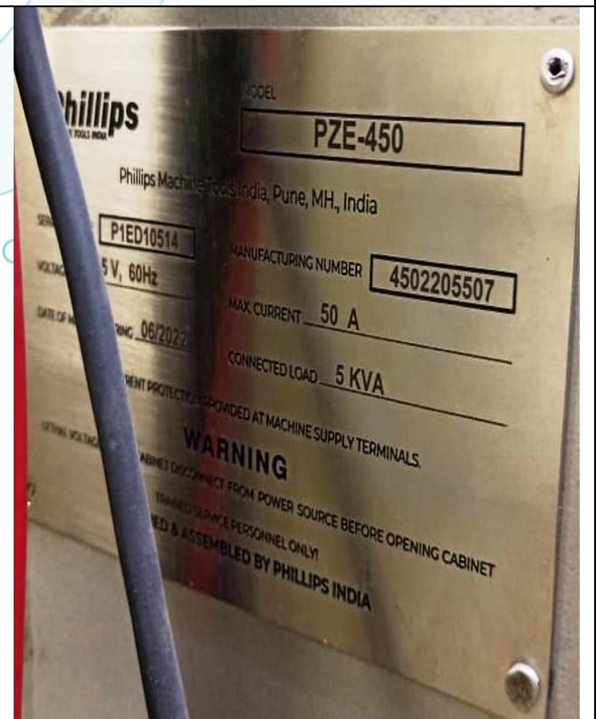
View of Phillips EDM Sinker ZNC, Model-PZE 450, Sr. No. P1ED10514
