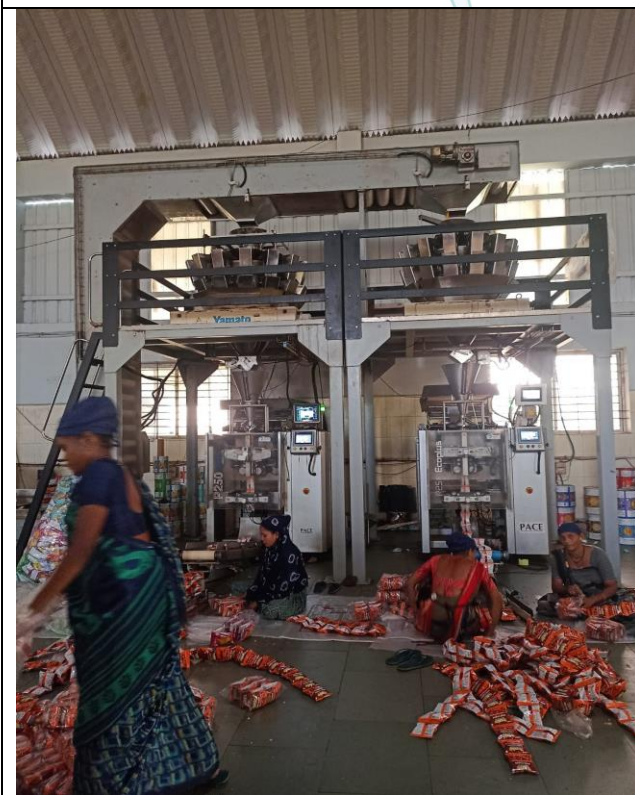
View of Pace Make High Speed Servo Driven Collar Type Vertical Form Fill Seal Machine with Accessories, Model No. P250 Eco+, Sr. No. SM-1769
