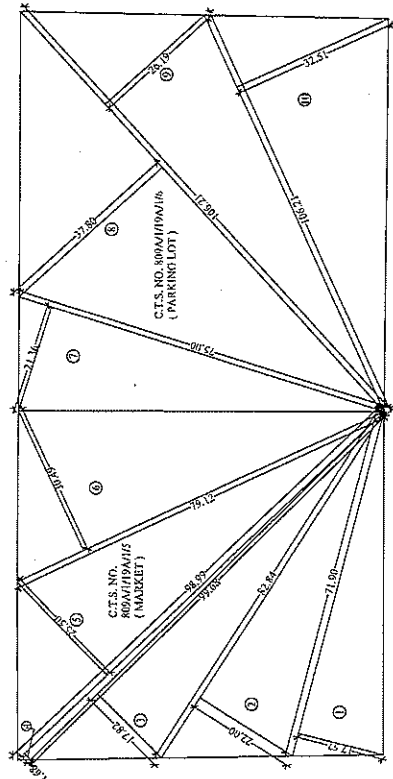
PLOT AREA LINE DIAGRAM (SCALE: 1:500)
