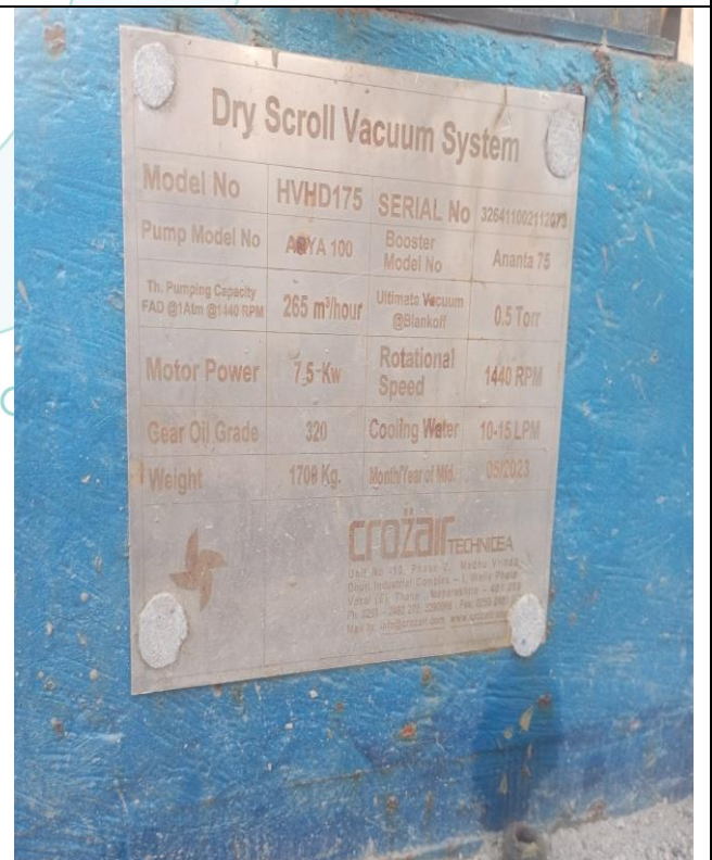
Dry Vacuum Pump
