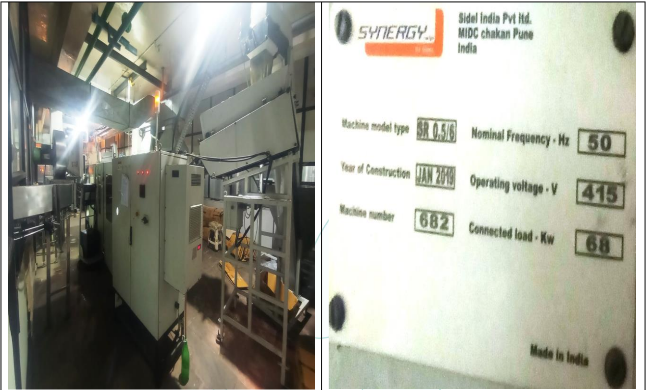
View of Synergy 0.5/6 Blowing Machine, Sr. No. 682
