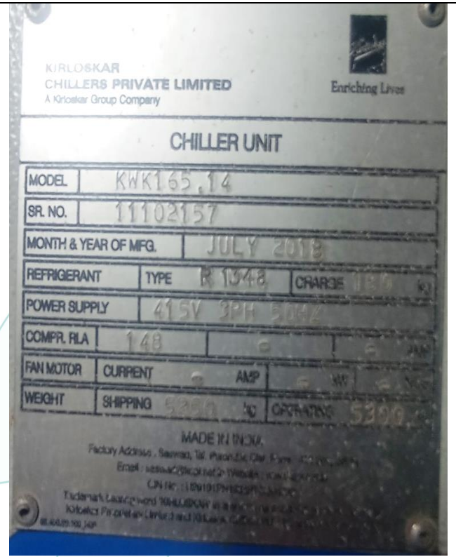
View of Water Cooled Screw Chiller, KWK165.14, Sr. No. 11102157
