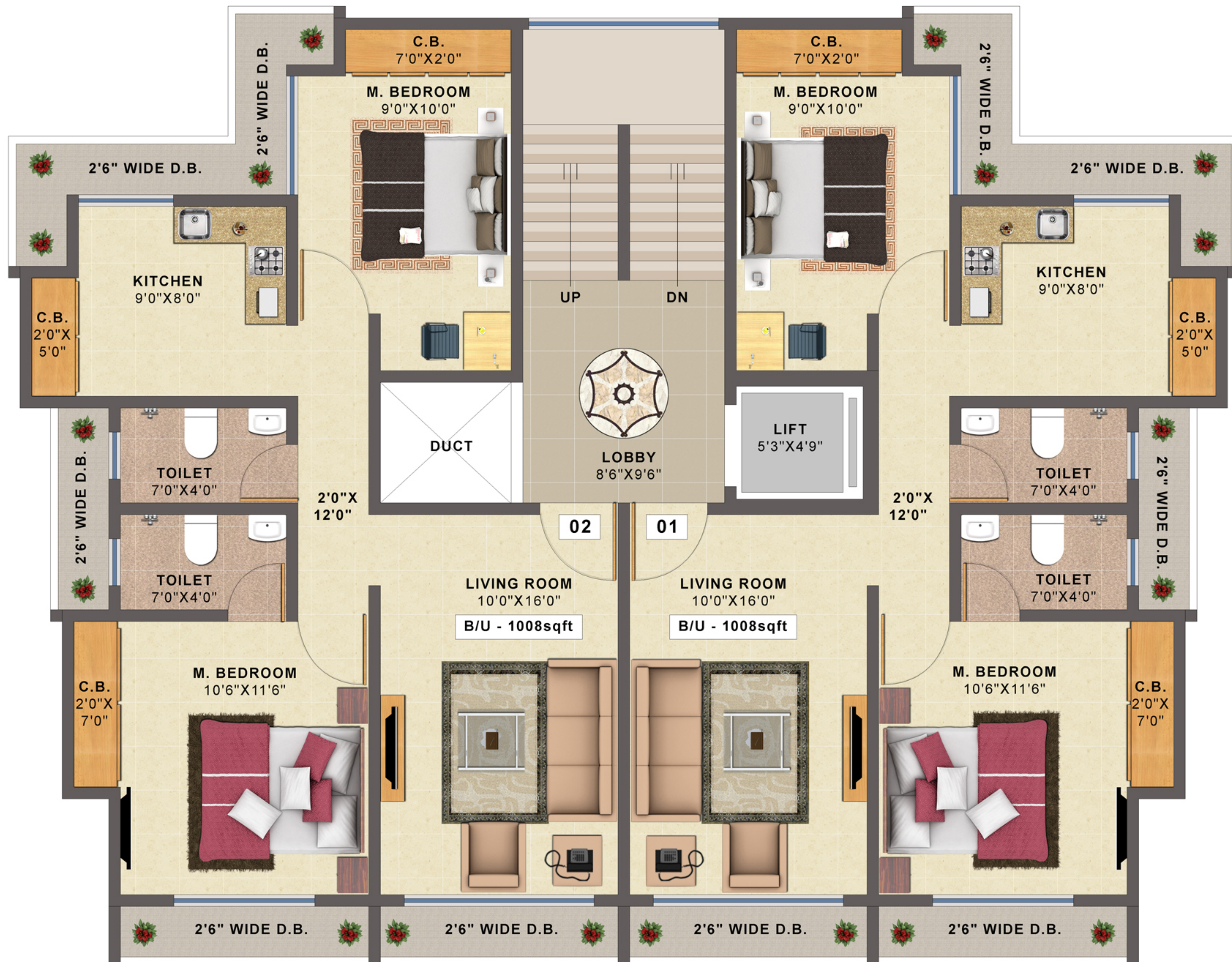
TYPICAL FLOOR PLAN 1ST TO 7TH FLOOR
