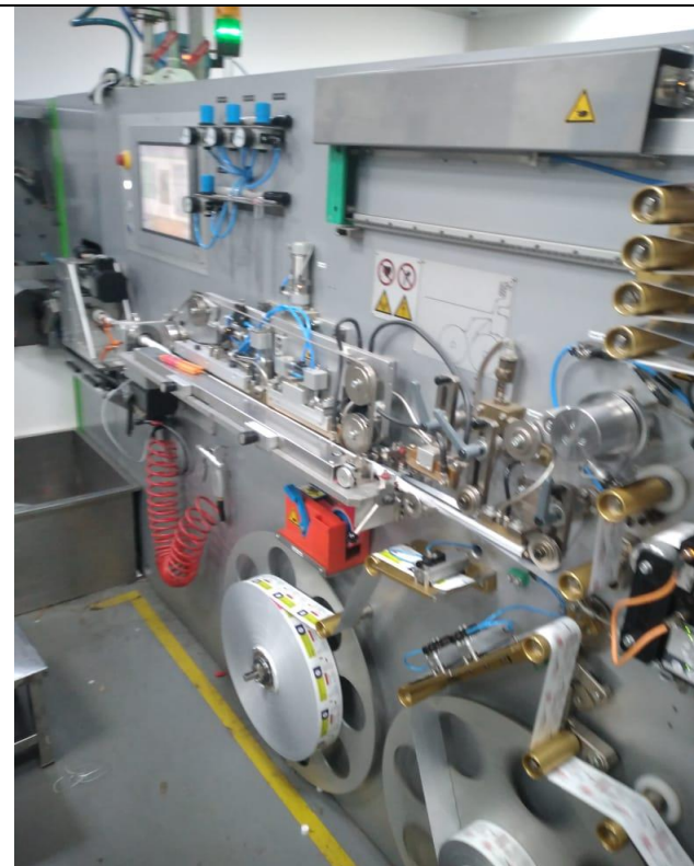
Laminated Tube Making Machine Mini 120 HF Fully Automatic Line
