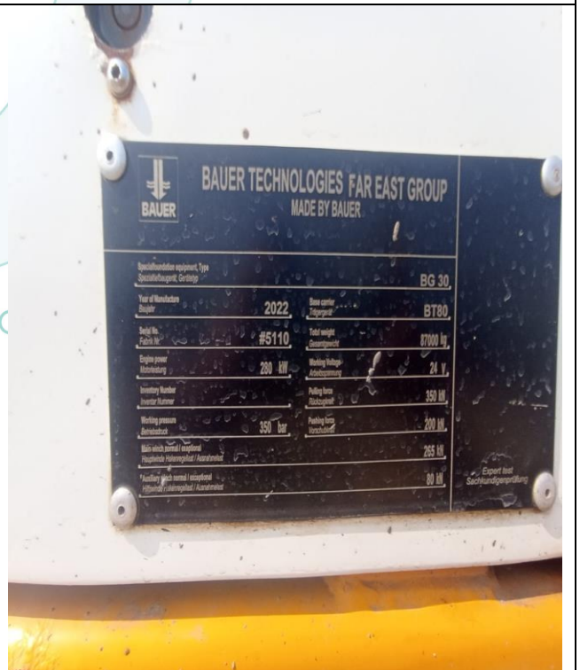
Bauer Rotary Drilling Rig BG 30, S/N: 5110
