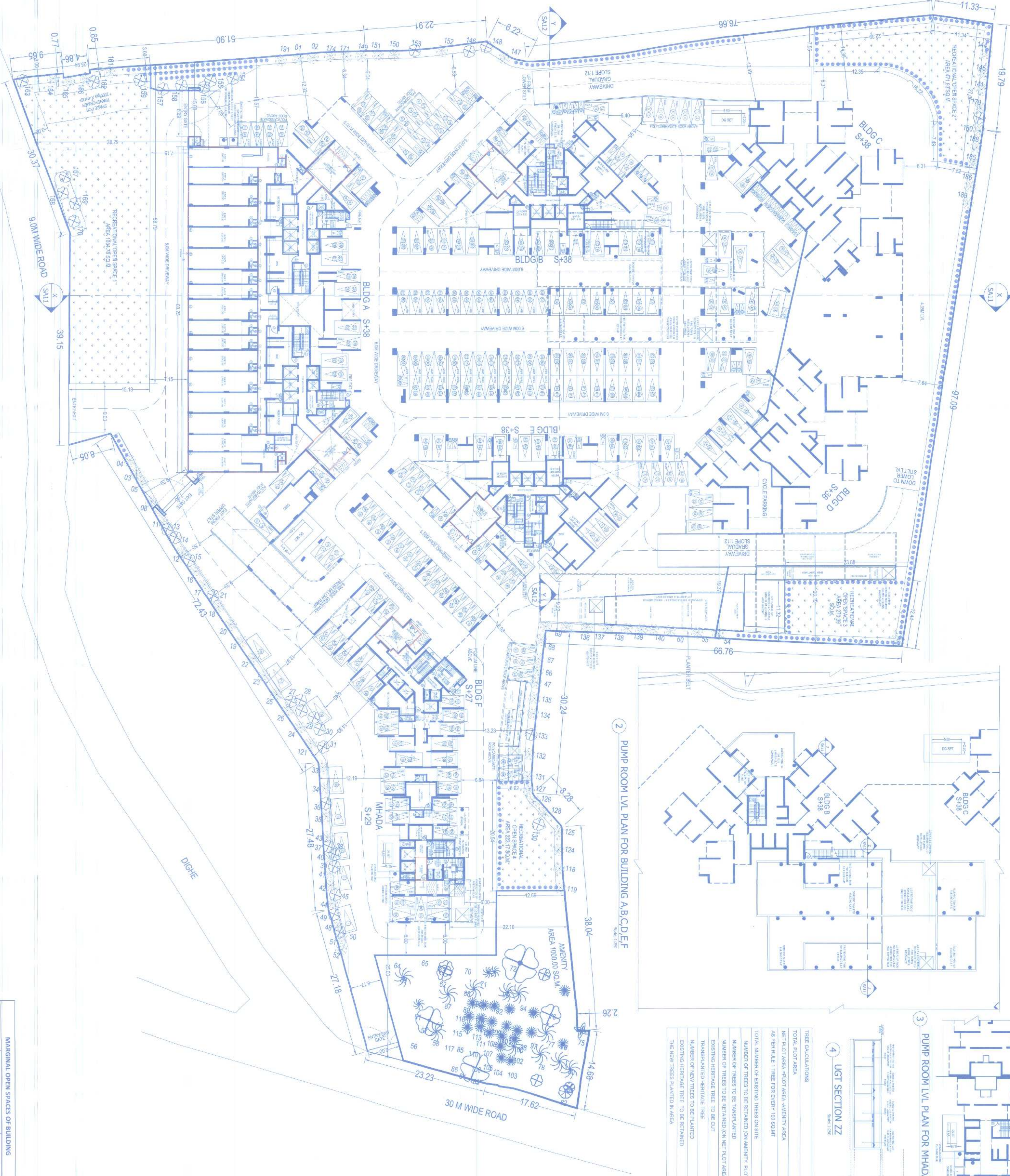
1 LOWER STILT LEVEL PLAN Scale: 1:250
