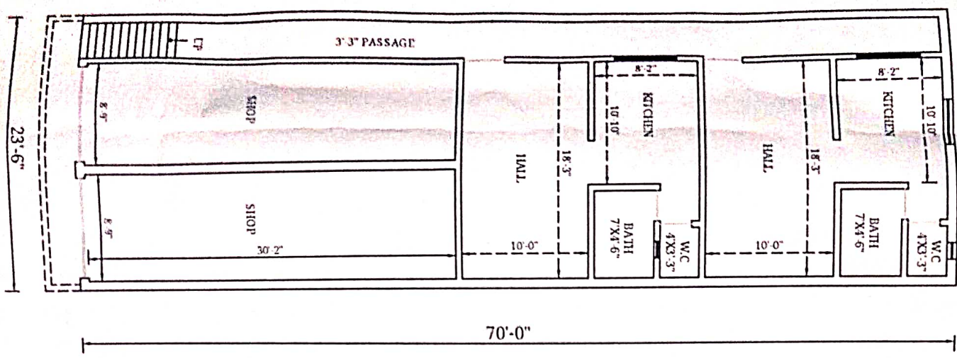
BASEMENT PLAN
