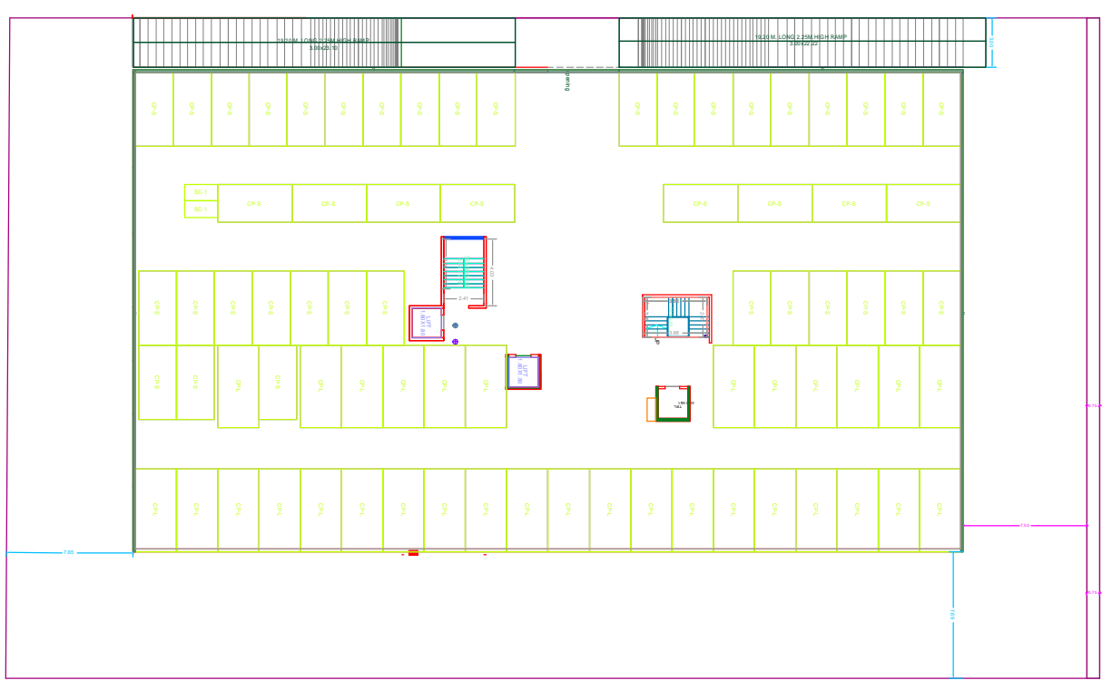
UPPER BASEMENT FLOOR PLAN SCALE: 1/100
