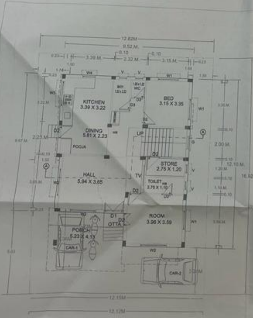
GR.FLOOR PLAN SCALE- 1:100
