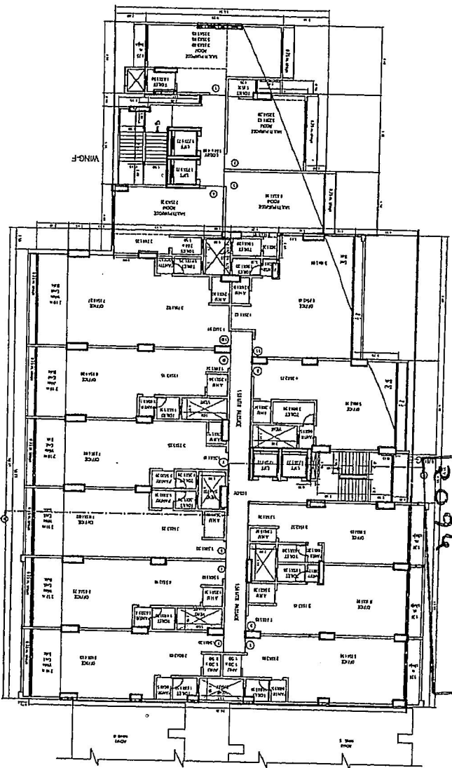
2ND TO 6TH, 8TH, 9TH FLOOR PLAN SCALE 1:100
