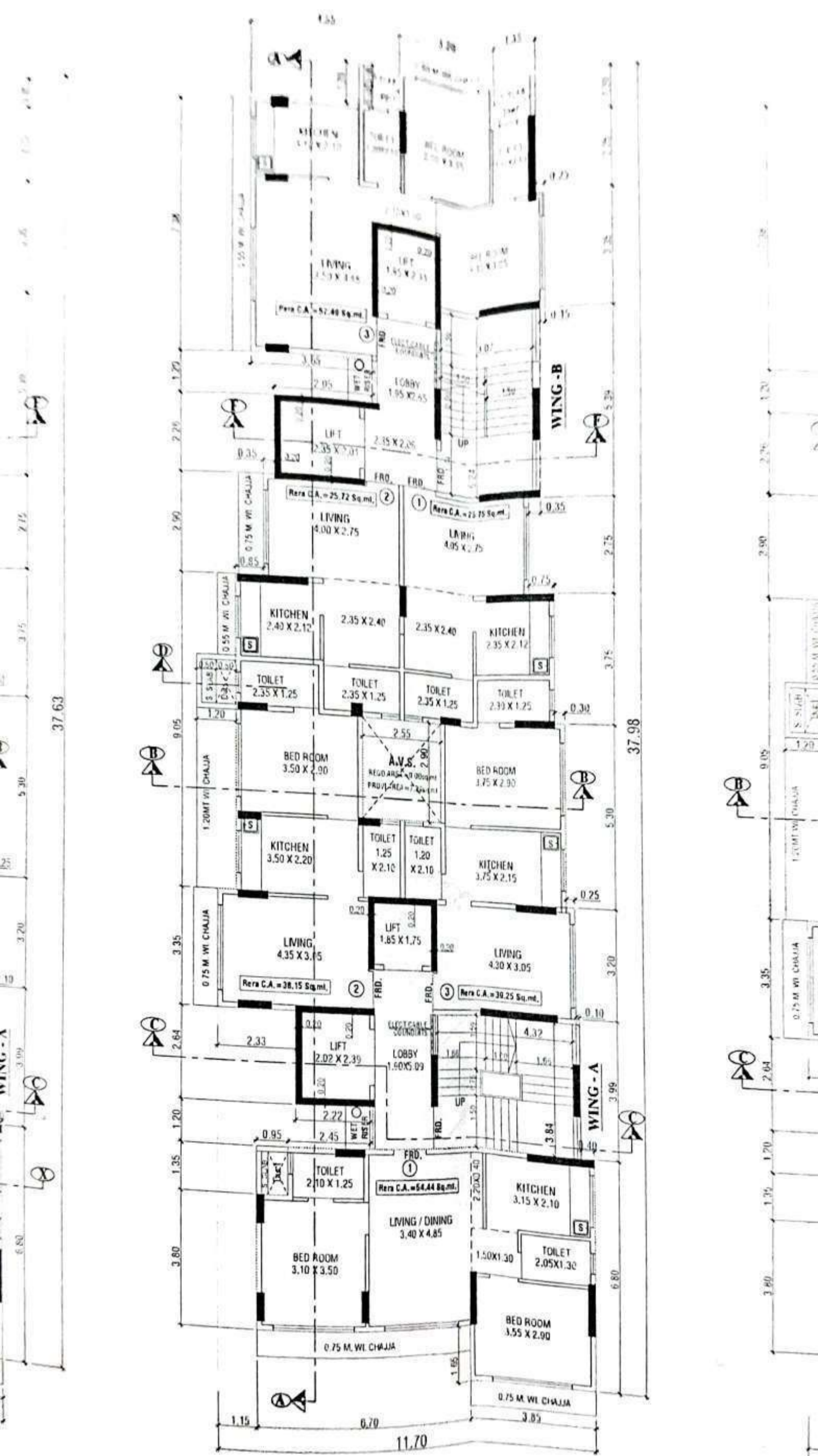
5th, 6th & 9th to 11th FLOOR PLAN SCALE - 1:100
