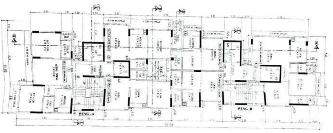
5th, 6th & 9th to 11th FLOOR PLAN SCALE - 1:100
