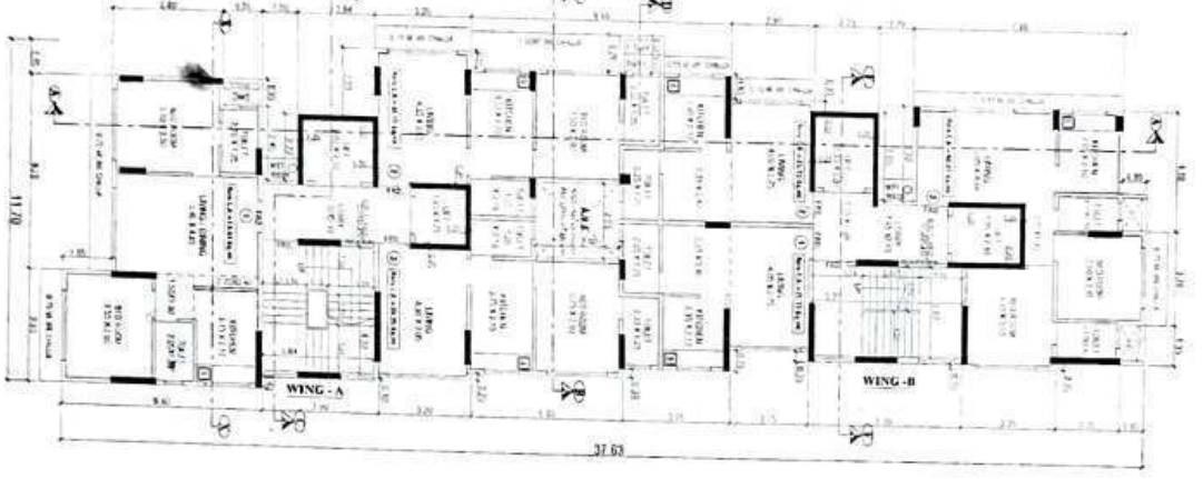
2ND TO 4TH FLOOR PLAN SCALE - 1:100
