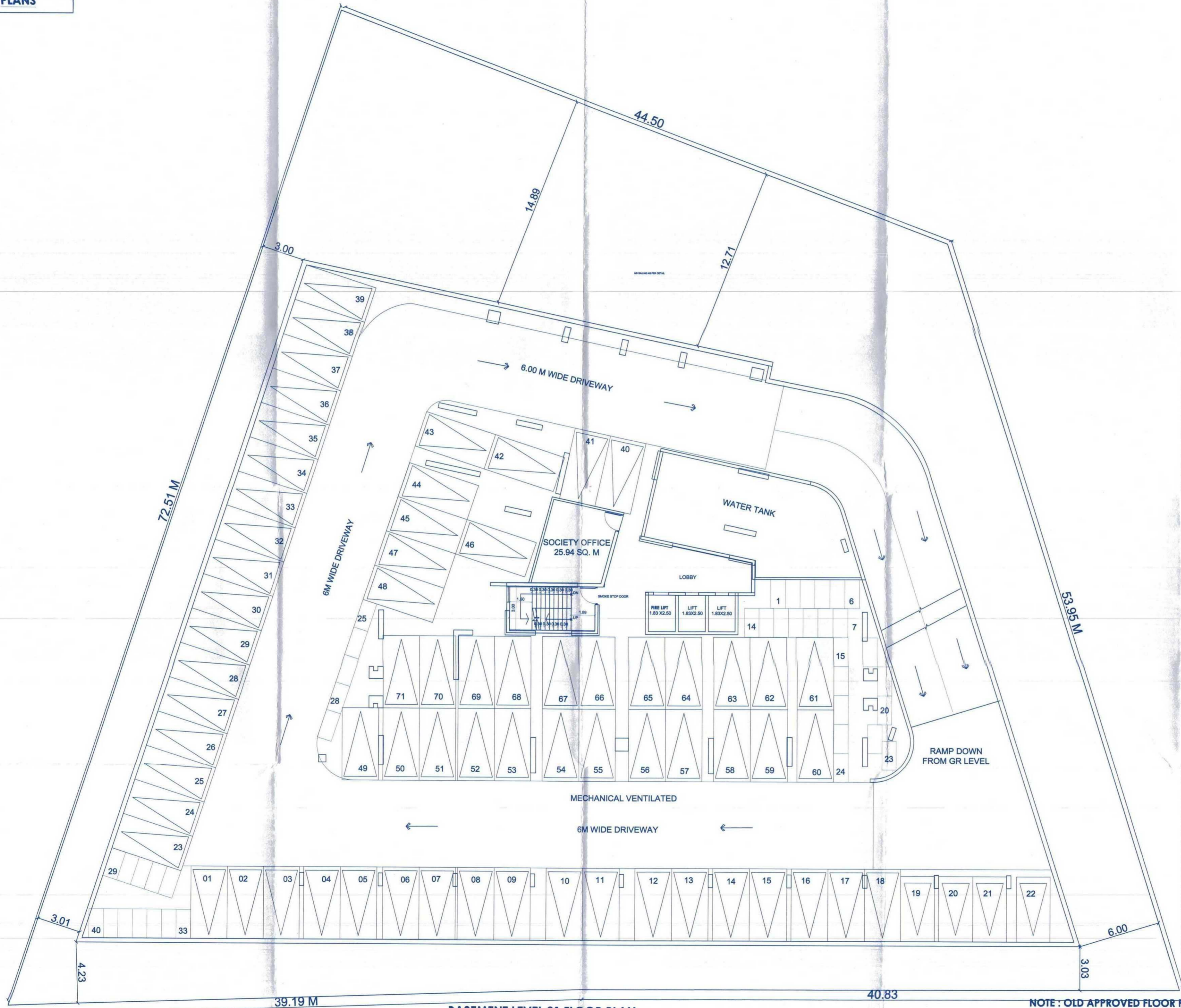
BASEMENT LEVEL 01 FLOOR PLAN
