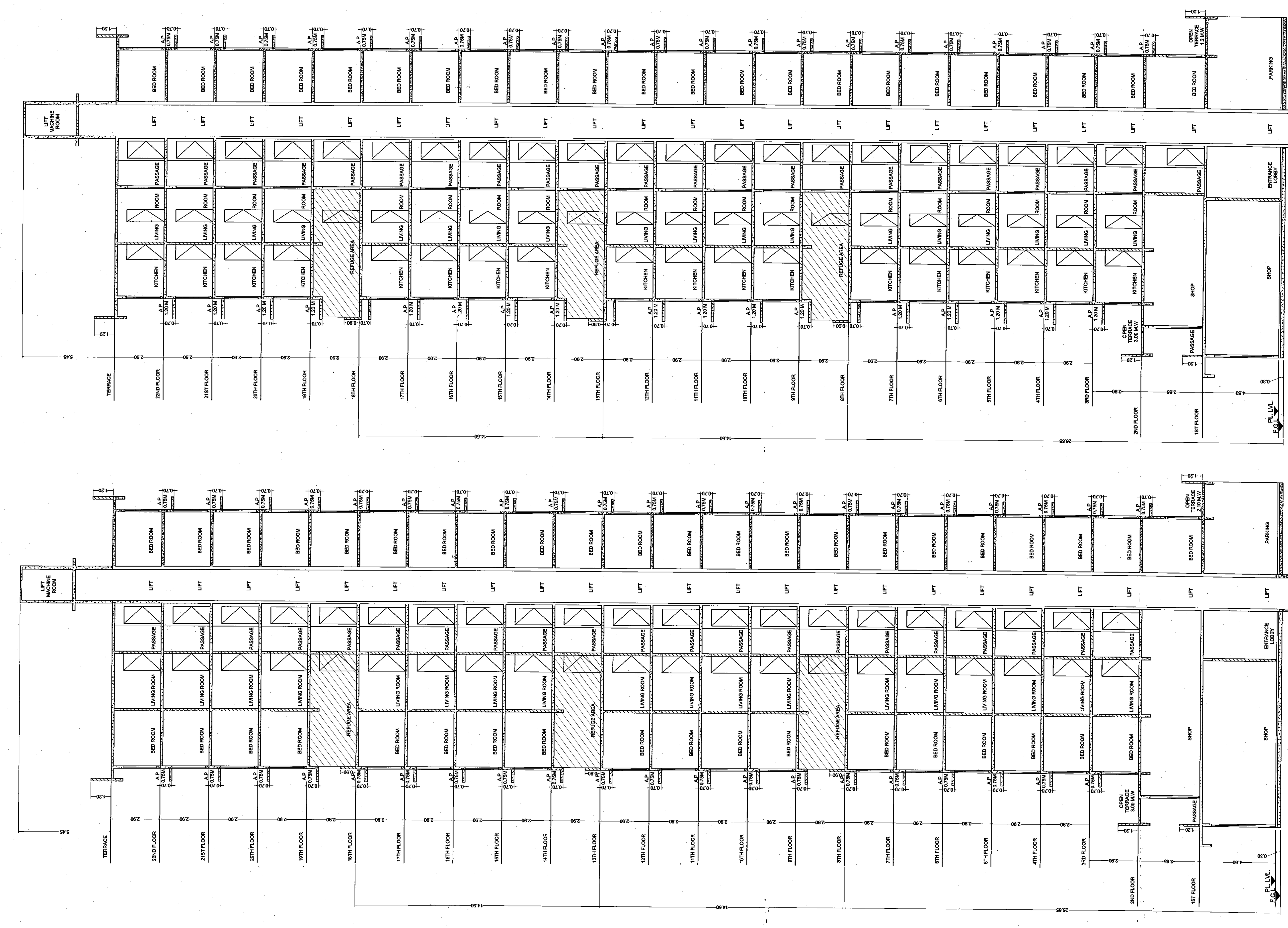
SECTION C-C OF B-WING OF BLDG NO. 01 SCALE 1:100
