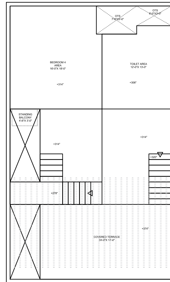
SF LAYOUT PLAN
