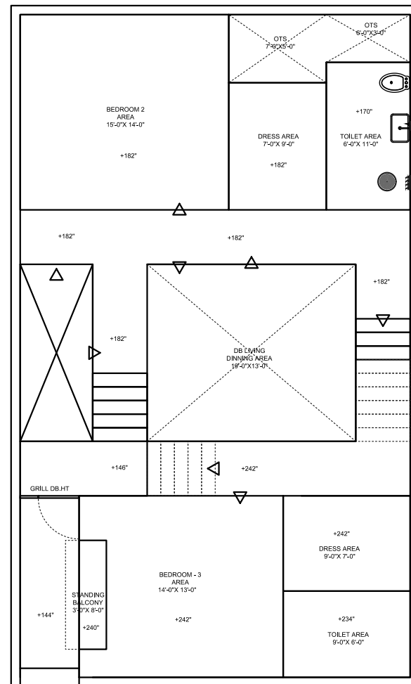
FF LAYOUT PLAN
