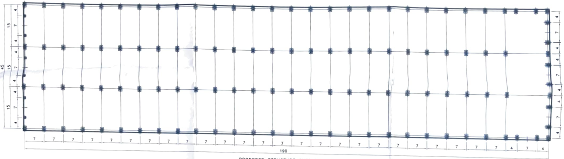
PROPOSED STRUCTURE SHED LAYOUT (SIZE IN METER = 45 x 190 METR.) (SIZE IN FOOT = 147.64' x 623.36' FOOT.)
