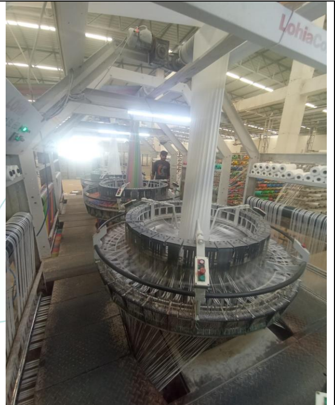
Circular Loom Model LSL6B
