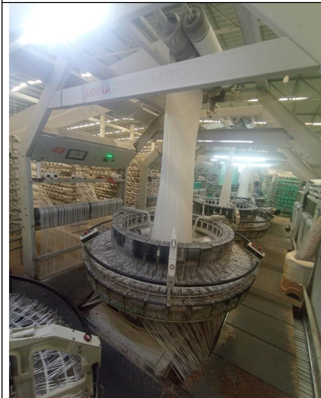
Circular Loom Model LSL6
