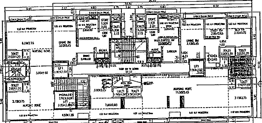
1ST FLOOR PLAN SCALE 1:100
