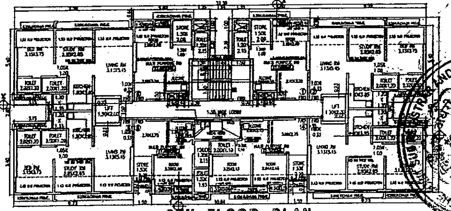
9TH FLOOR PLAN SCALE 1:100
