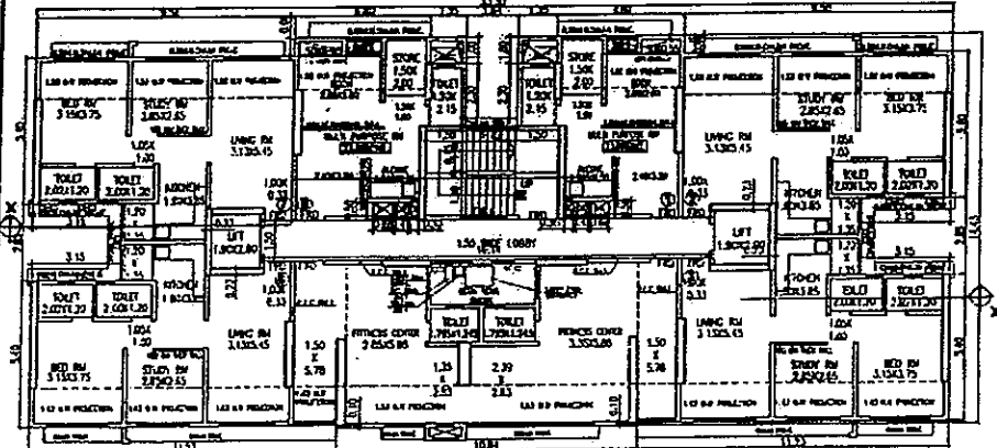
2ND FLOOR PLAN SCALE 1:100
