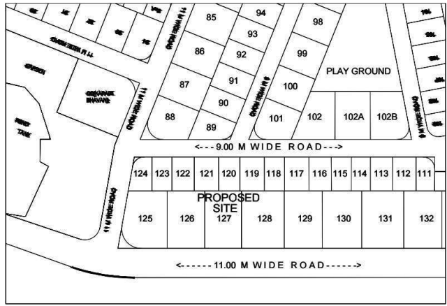
PLOT NO.-127, SECTOR-R2, PUSHPAK, NAVI MUMBAI. LOCATION PLAN SCALE = 1:250
