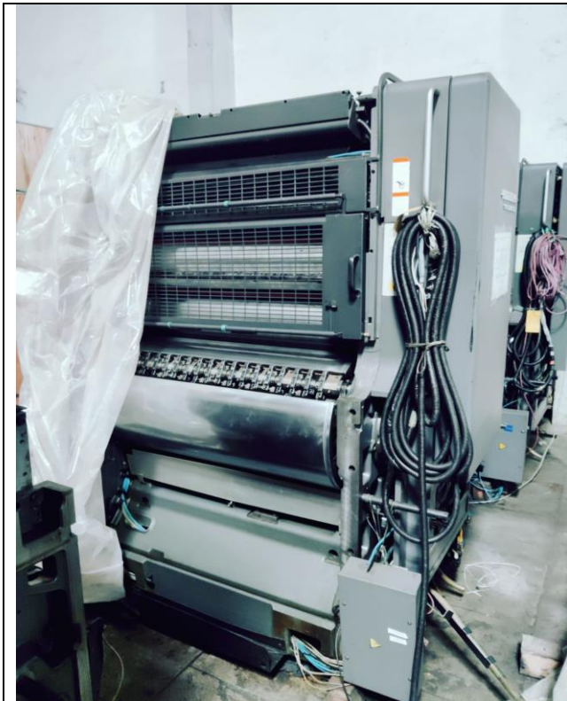
View of Used Heidelberg CD 102-6+L Printing Machine
