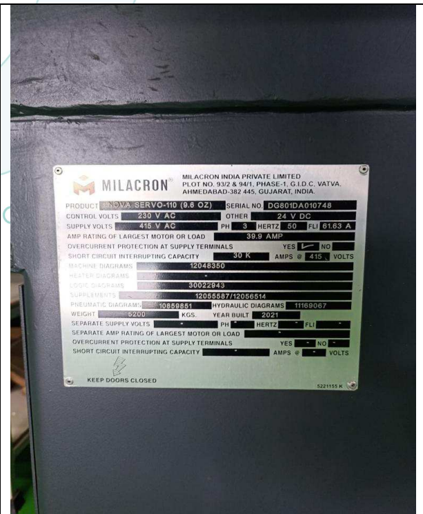
Machine Name Plate
